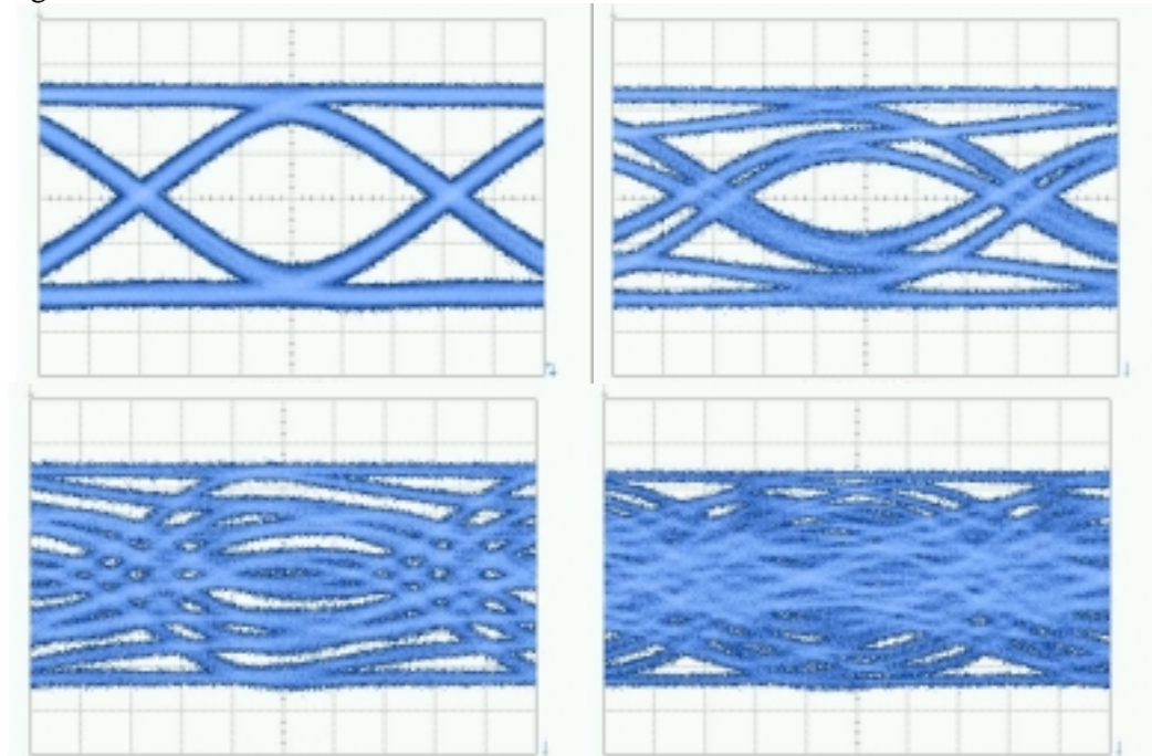
Fig. 1: Eye Diagrams Of 300 m Multimode Fibers Varying Bandwidths/DMD Profiles
