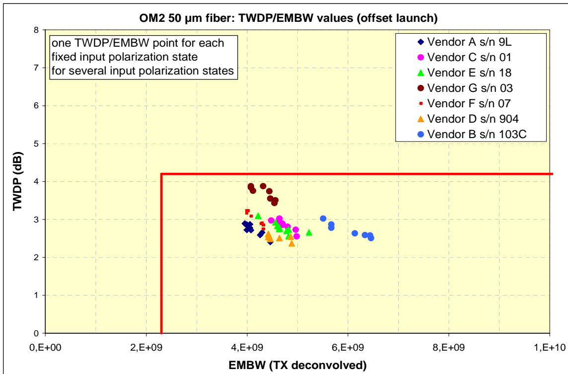
Fig. 4: TWDP/EMBW Values Over 260 m of OM2 Fiber (Offset Launch)
