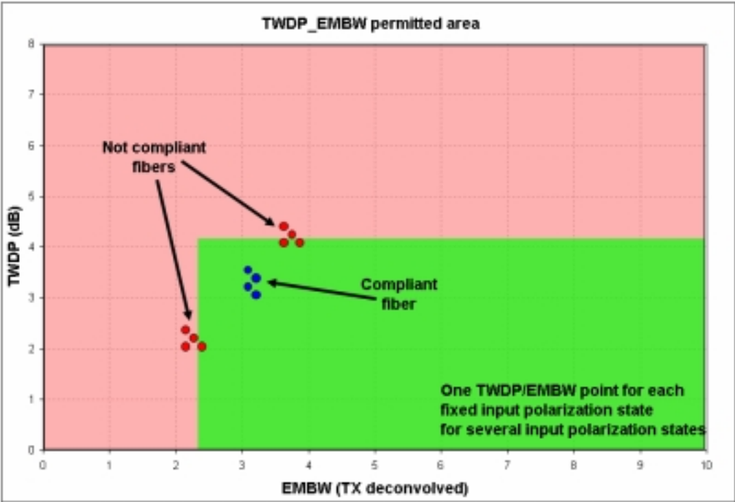
Fig. 2: TWDP/EMBW Permitted Area For 10GBASE-LRM-Compliant Fiber
