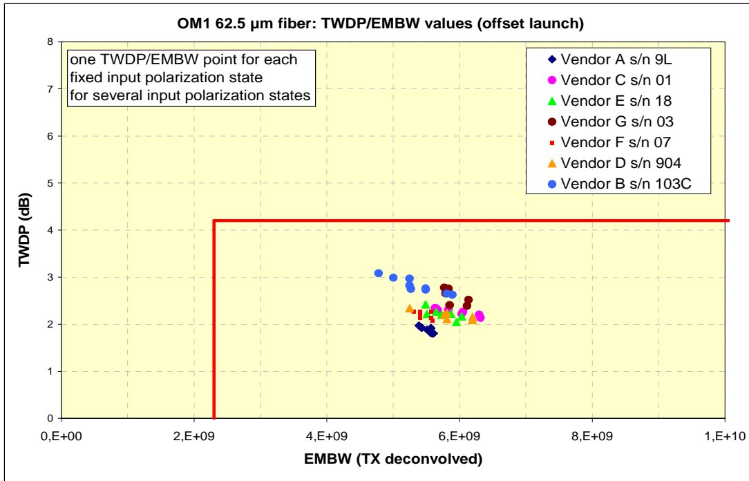
Fig. 3: TWDP/EMBW Values Over 216 m Of OM1 Fiber (Offset Launch)
