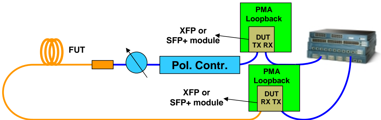
Fig. c: Traffic Test: XFP (SFP+) Transmitter - SFP+ (XFP) Receiver
