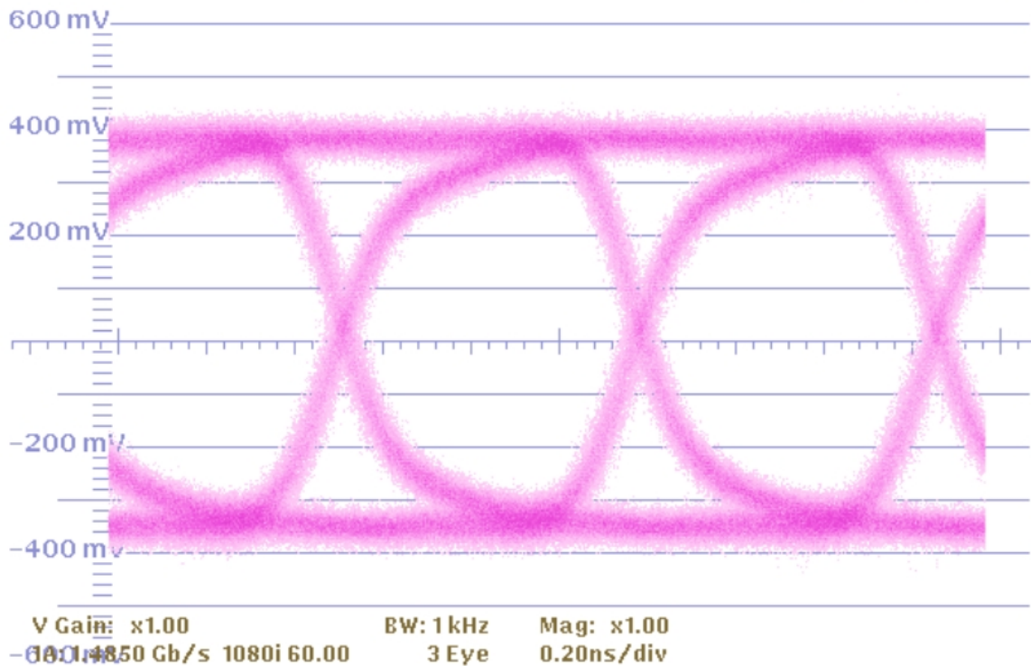
Fig. 5: HD-SDI output eye-diagram (obtained from Cypress Semiconductor's HOTLink II transceiver serial output using a Tektronix WFM700M waveform monitor)
