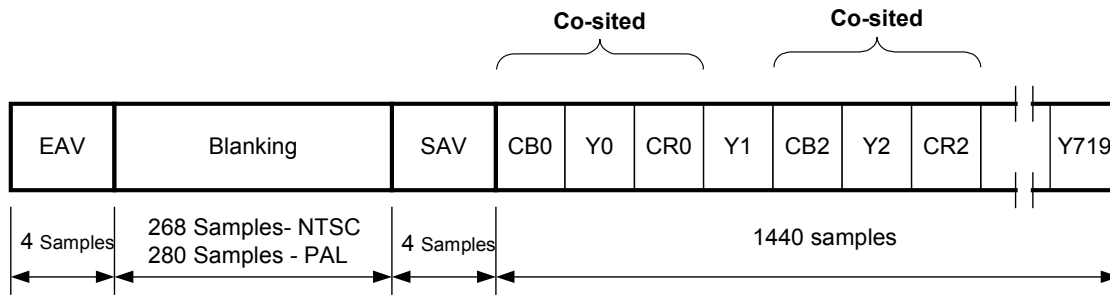
Fig. c: Data structure for each digital video line for 4:2:2 component digital video
